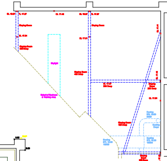
Ceiling Detail Above Business Centre & Training Room
