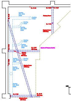
Ceiling Detail Above Finance Centre
